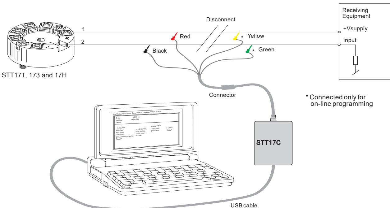
Figure 1-1 Connection using EZ-Mini-Hooks
