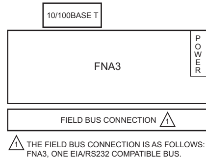
Fig. 2. FNA3 Components.
