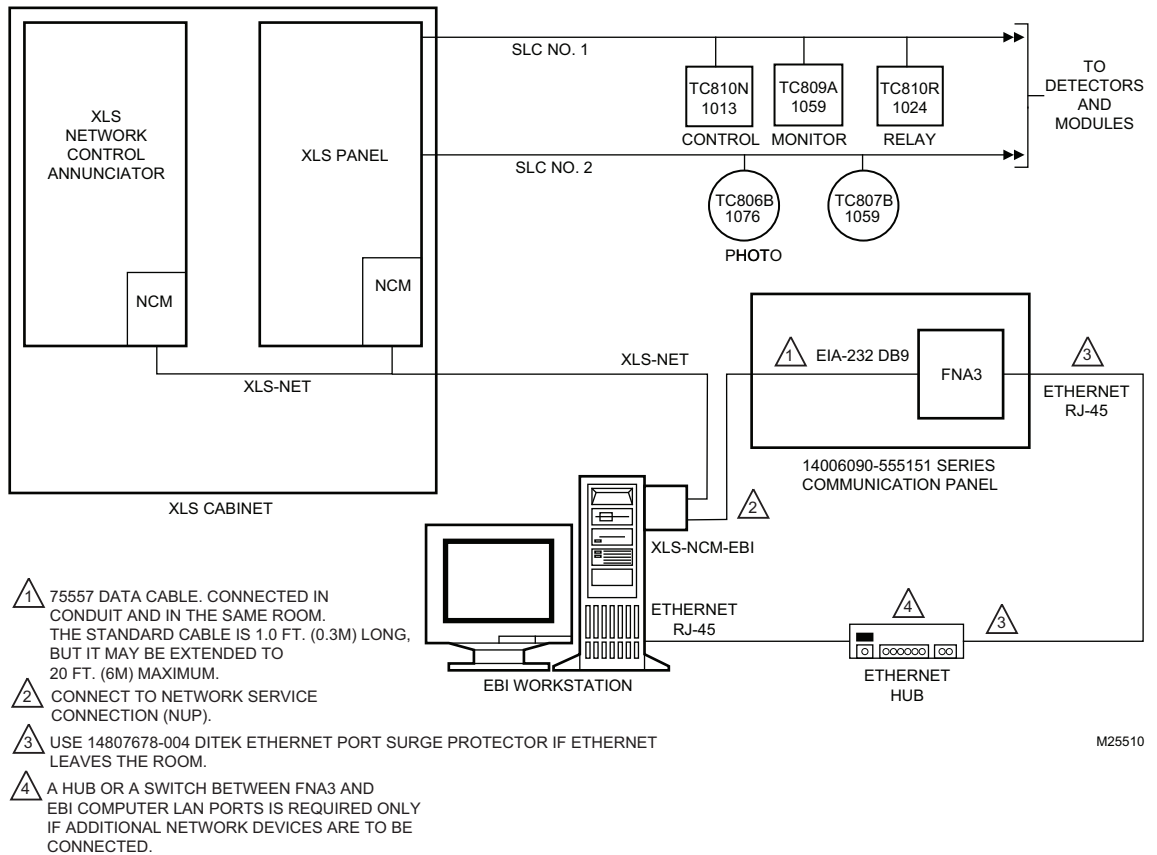
Fig. 8. Typical FNA3/XLS-NCM-EBI Connect Application Block Diagram.
