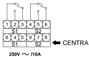
Auxiliary Switches
