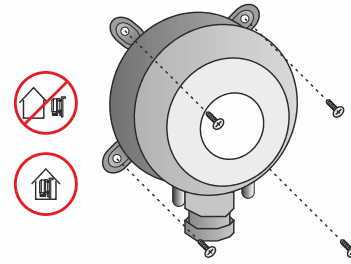
Fig. 2. Mounting
